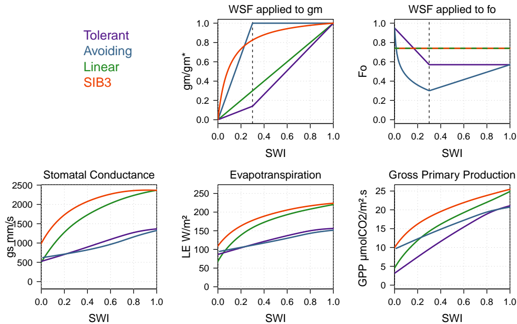
Figure 1. Graphical representation the mesophyll conductance ( g_m ), the coupling factor at saturating air humidity ( f_0 ), the stomatal conductance ( g_s ), the evapotranspiration (LE) and the gross primary production (GPP) for the four water stress functions (WSF) used in this study against the soil wetness index (SWI).
