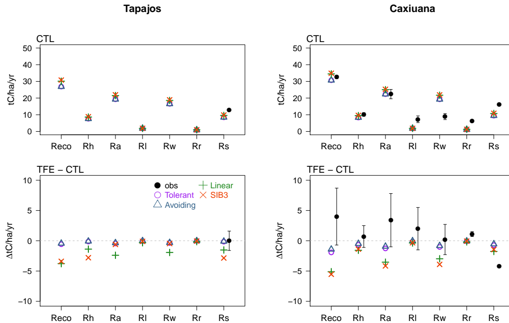
Figure 8. Annual ecosystem ( R_{ECO} ), heterotrophic ( R_H ), autotrophic ( R_A ), leaf ( R_l ), wood ( R_w ), root ( R_r ) and soil ( R_s ) respirations for the fourth year of the experiment for the control plot (top) and the difference between the exclusion and control plot (bottom) at Tapajós (left) and Caxiuanã (right).
