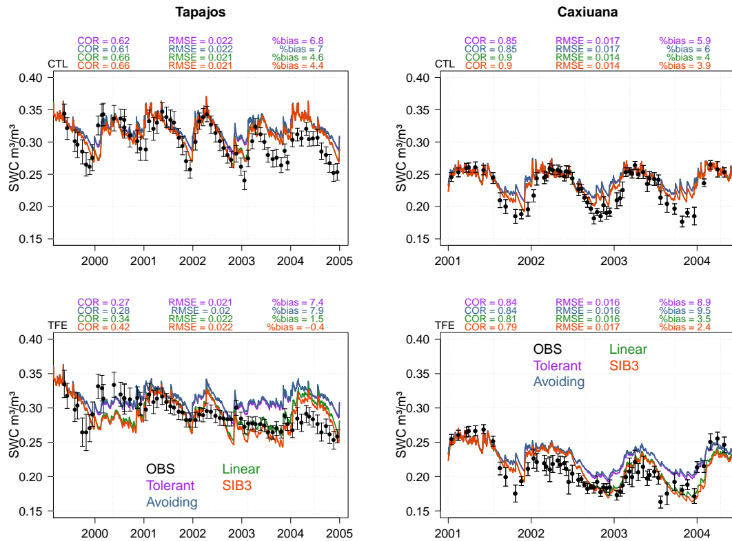
Figure 3. Daily observed and simulated soil water content with the four water stress functions (WSFs) at Tapajós (left) and Caxiuana (right) for both control (CTL) (top) and throughfall exclusion (TFE) (bottom) plots. The soil water content (SWC) measured at the TFE plots were rescaled to have the same SWC as that of the CTL plots during the baseline year.
