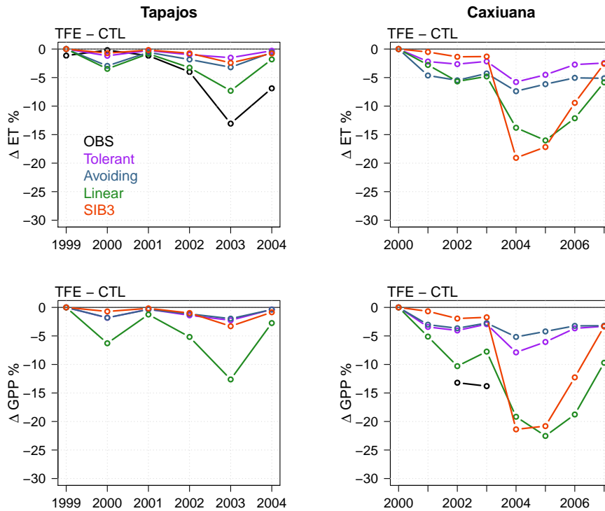
Figure 7. Annual mean differences (throughfall exclusion (TFE) plot minus control (CTL) plot) in simulated evapotranspiration (ET) (top) with ISBA CC and Markewitz's model outputs as a proxy (Markewitz et al., 2010). Annual differences (exclusion plot minus control plot) in simulated gross primary production (GPP) (bottom) with ISBA CC and SPA's model outputs as a proxy (Fisher et al., 2007).
