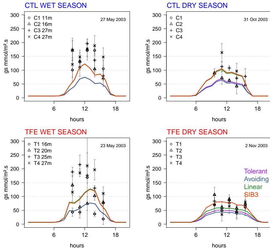
Figure 6. Seasonal variability of the diurnal cycle of stomatal conductance at Caxiuana. Measurements were taken on 4 days at four different heights in the canopy: C1–C4 designate trees in the control (CTL) plot and T1–T4 trees in the throughfall exclusion (TFE) plots and simulated g_s with the four water stress functions (WSFs) (lines) are representing all canopies.
